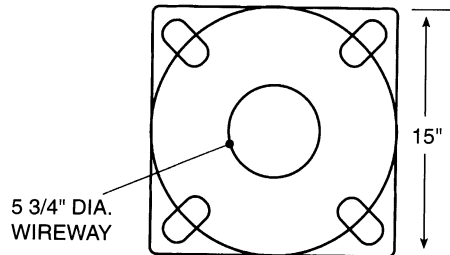
TOP PLAN
